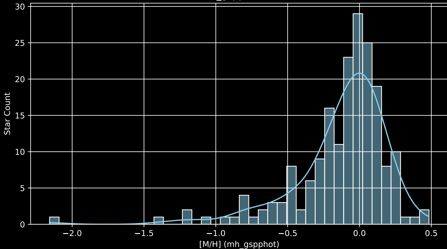
APOGEE DR17 Field: [105+12 [M/H] (mh_gspphot) (n= 190)
