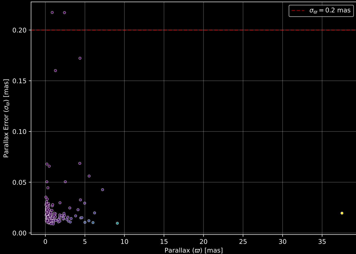
APOGEE DR17 Field: [105+12] Parallax Quality (n= 194)
