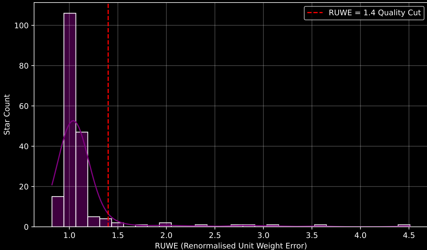
GAPOGEE DR17 Field [105+12] RUWE Distribution (n= 188)
