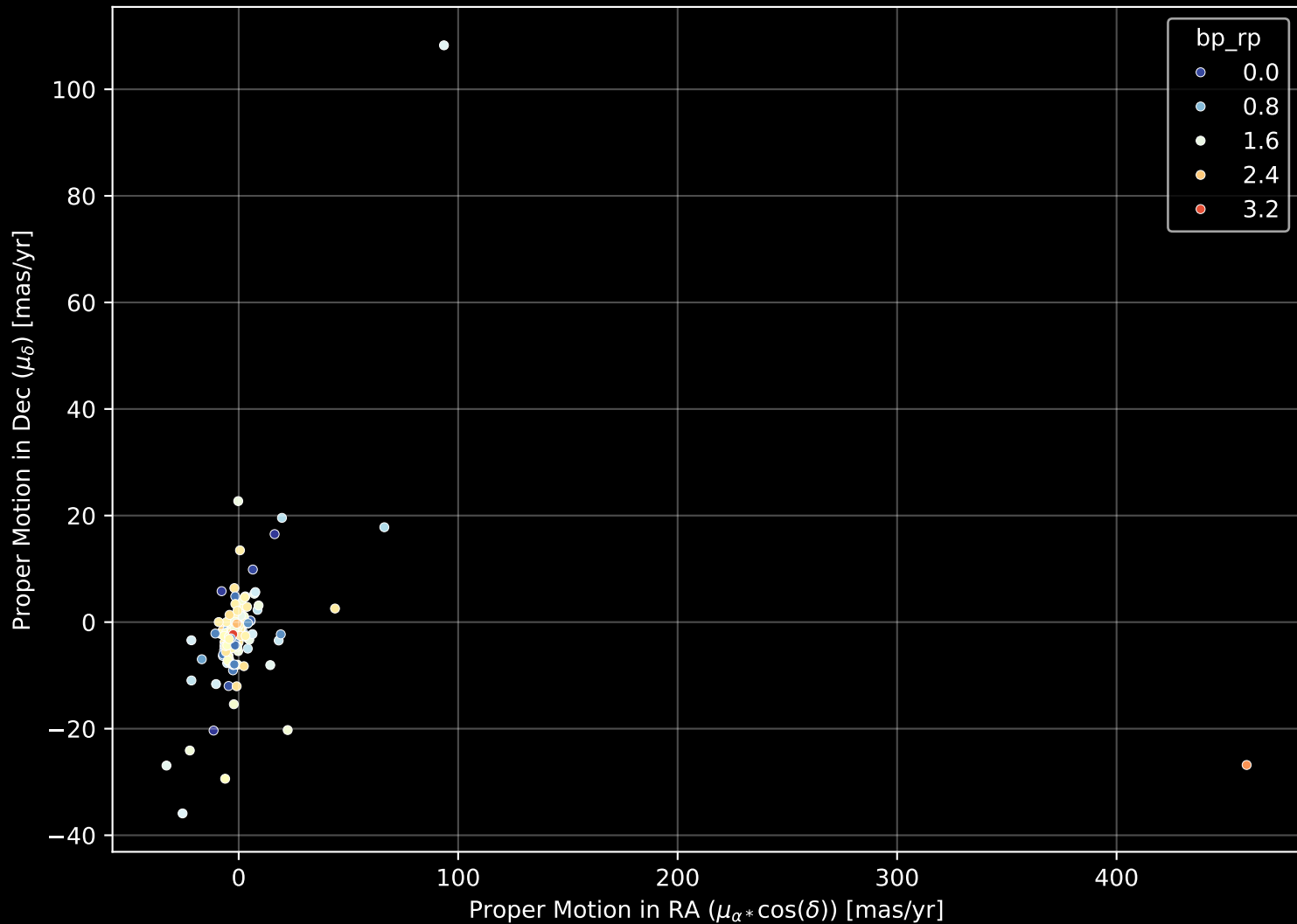
APOGEE DR17 Field: [105+12] Proper Motion Diagram (n= 194)
